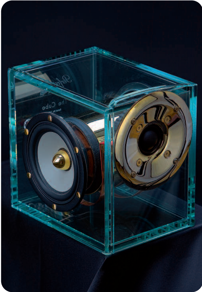
▲ THE CUBE front loudspeaker
